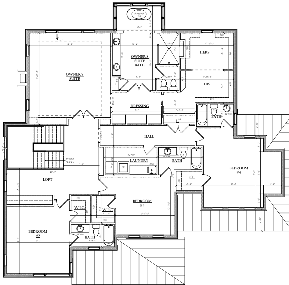
1 2 3 4 5 6 7 8 9 10 A B C D E F G H I J SECOND FLOOR PLAN SCALE: 1/4" = 1'-0"
