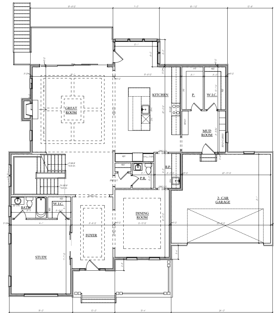
1 GROUND FLOOR PLAN A.02 SCALE 1/4" = 1'-0"
